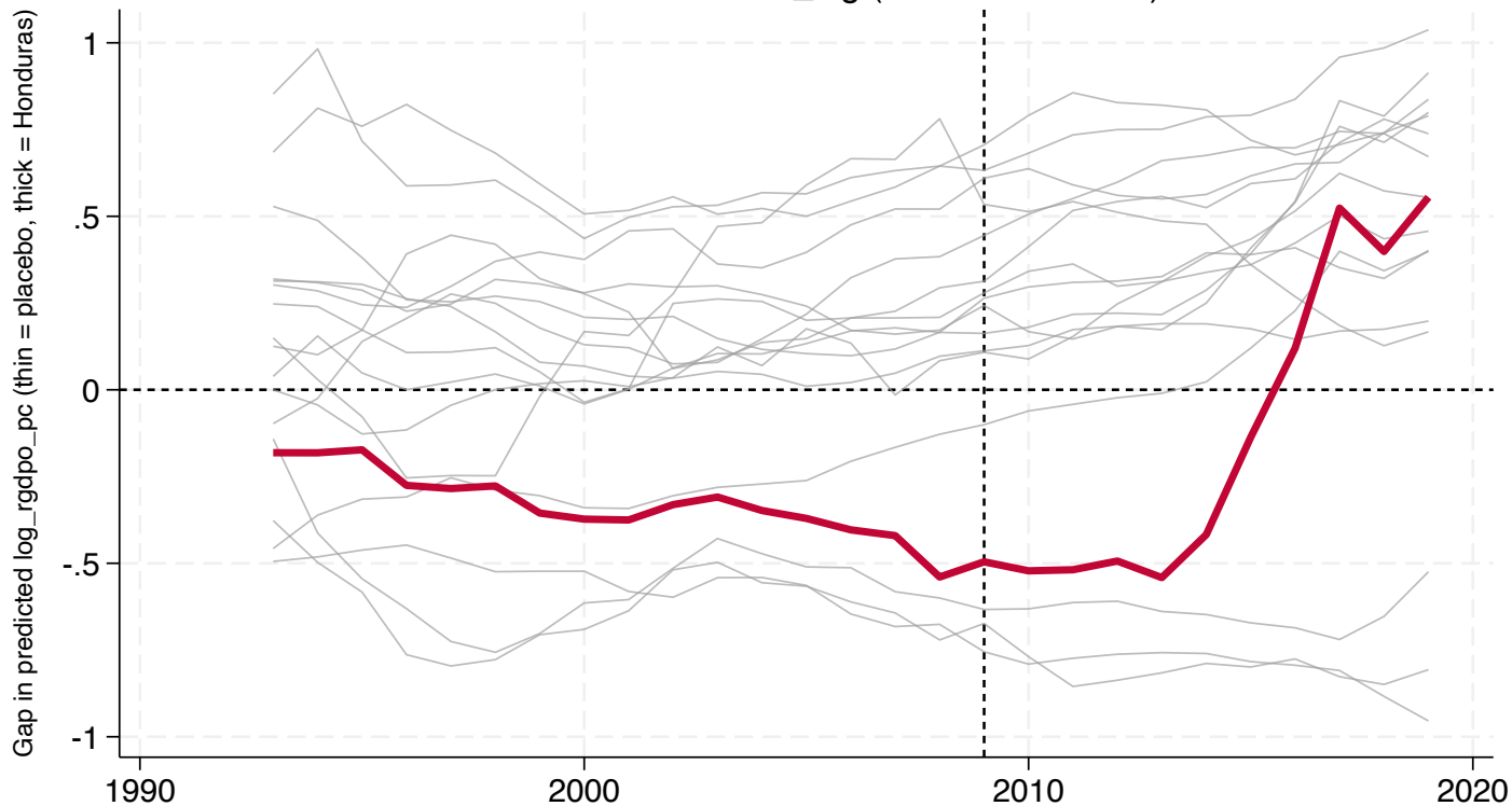
Latin America: factors_log (outliers excluded)
